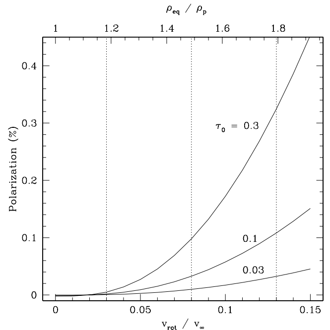
FIG. 13.—Continuum polarizations arising from Thomson scattering of starlight in the mildly distorted WCZ models. The abscissa is v_{\text{rot}}/v_{\infty} , relevant for the models presented in this paper. Also shown at top is the corresponding asymptotic equator-to-pole density contrast. The electron scattering is assumed to be optically thin, with envelope optical depths \tau_0 as indicated. These \tau_0 values are for an equivalent spherical envelope. The continuum polarizations are for an edge-on view and will scale as \sin^2 i for other viewing inclinations. The vertical dotted lines indicate the corresponding models used in the line calculations for the WCFields magnetic geometry assuming a spherical wind density.
