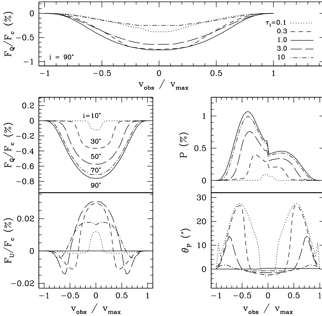
FIG. 11.—Series of polarized line profiles for a WCFields model with v_{\text{rot}} = 0.08v_{\infty} to highlight the influence of optical depth and viewing inclination effects. The surface field strength is B_* = 10B_{\text{Han}} for every profile. The top panel shows the continuum normalized Q -flux for i = 90^\circ , with the line optical depth varied as indicated. The four panels below show the influence of viewing inclination for \tau_l = 1.0 . Left panels: Plots of F_Q/F_c and F_U/F_c in percent polarization. Right panels: Plots of P (this being normalized to the full P Cygni line profile and not just the continuum level) and \theta_p . The different curves are for the inclination values shown in the panel for F_Q .
