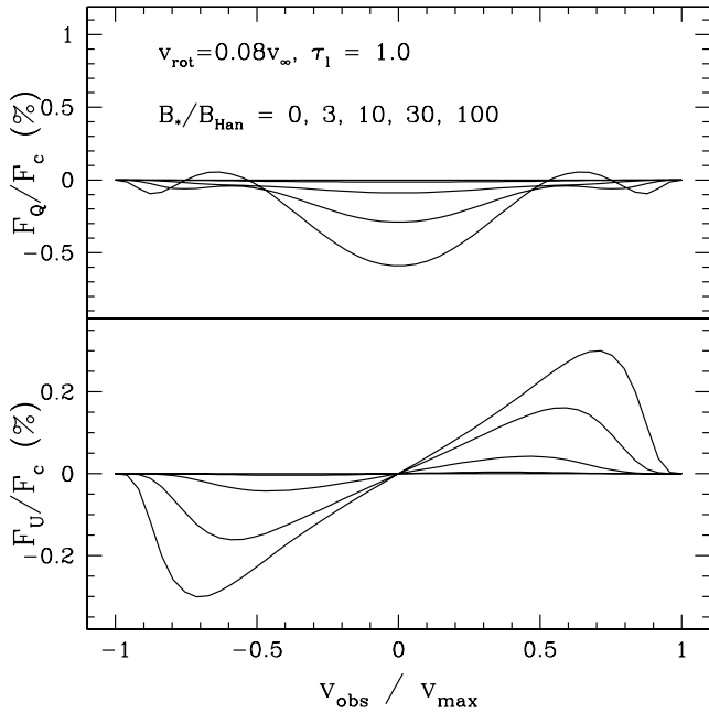
FIG. 14.—Polarized line profiles in Q and U for a WCFields model, with v_{\text{rot}}/v_{\infty} = 0.08 and a spherical density, but with an initial magnetic field at the wind base that is a magnetic monopole. Compared to the basal split monopole configuration used in Fig. 9, the Q -polarization has dropped, and a significant and antisymmetric U -profile is now evident. Consequently, the U -profile, when the polarization measurement axis is aligned with the source symmetry axis, is sensitive to the symmetry of the circumstellar magnetic geometry.
