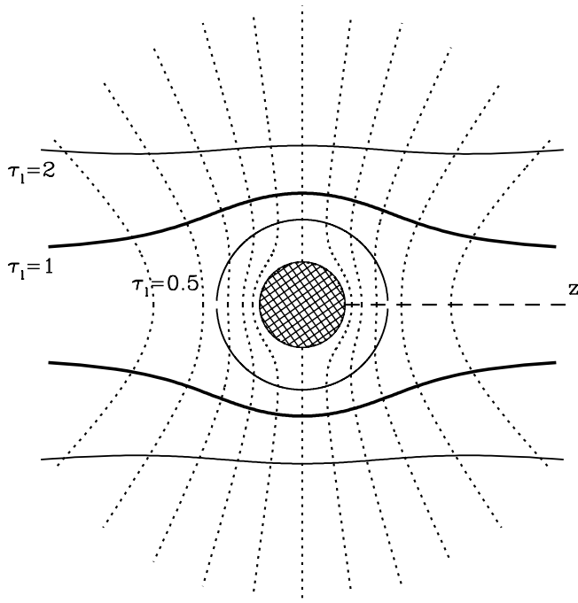
FIG. 7.—Isovelocity zones ( dotted lines ), with the observer to the right. The solid lines demarcate regions of the wind where the Sobolev optical depth in the line is thick ( \tau_S > 1 interior to the curves) and thin ( \tau_S < 1 exterior to the curves). Three cases are shown, with \tau_1 = 0.5, 1 , and 2 . The \tau_1 = 1 case is shown as a thick line, since it is the value adopted for most of our line calculations. In this particular case, some portion of every isovelocity zone is optically thick in the line. In the single-scattering approximation, polarized line emission is produced only at locations where \tau_S < 1 .
