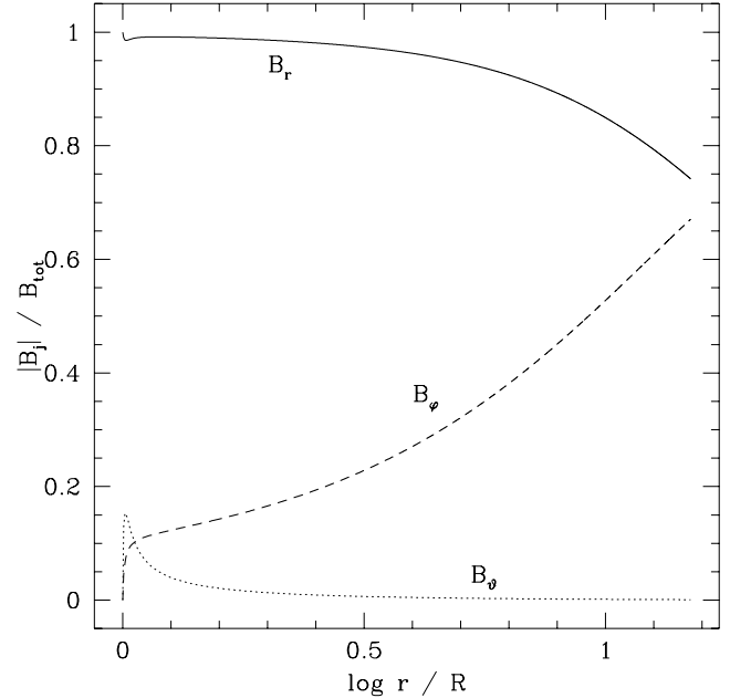
FIG. 10.—Variation of the magnetic field components from the WCFields model as a function of radius, using approximations that apply for slow stellar rotations. The individual components are normalized to the local total magnetic field strength. These curves are for the case v_{\text{rot}}/v_{\infty} = 0.08 at a latitude of \vartheta = 45^\circ so as to roughly maximize the contribution of the latitudinal component B_\vartheta .
