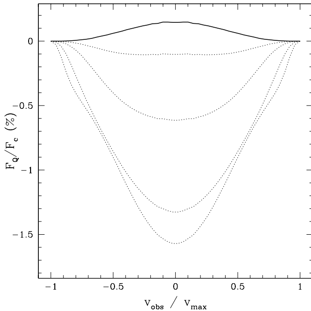
FIG. 12.—Hanle effect for a WCFields model with v_{\text{rot}}/v_{\infty} = 0.08 but with an aspherical wind. The solid line shows the line polarization that results when there is no magnetic field. The dotted lines are with the Hanle effect (to be compared with Fig. 9, middle ). The view is edge-on, and \tau_1 = 1 for all of the profiles. For B = 0 , peak polarization occurs near line center and is positive because there are relatively more line scatterers in the vicinity of the equator than near the poles.
