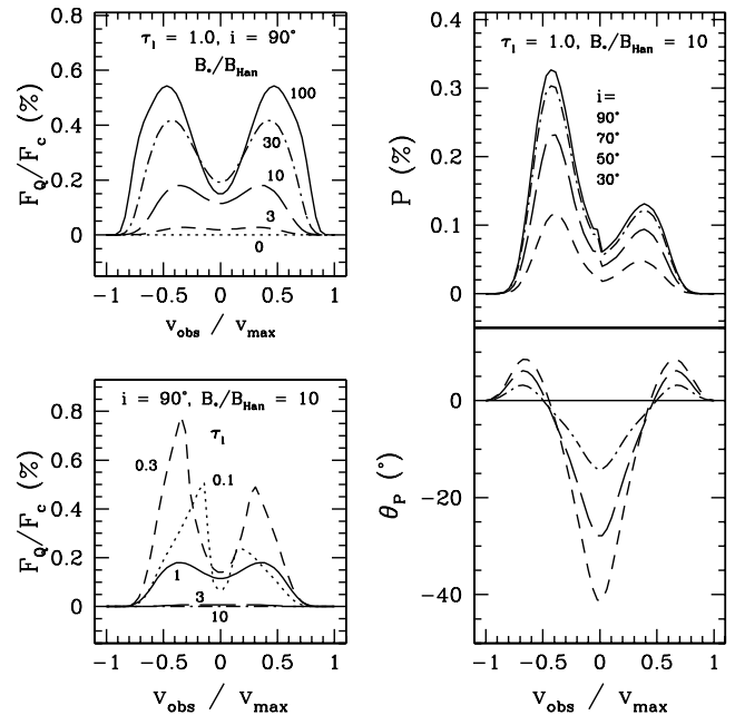
FIG. 8.—Percent polarization of the Hanle effect for a dipole magnetic field in a spherical stellar wind. Top left : Polarized Stokes Q -profiles as normalized to the continuum emission outside the line frequencies. For a dipole field as seen from the side in a line with \tau_1 = 1.0 , larger Hanle ratios (as labeled) yield higher line polarizations. Bottom left : As in the top left panel, except with \tau_1 varied as indicated for a fixed Hanle ratio. Note that the line asymmetry for the two lower optical depth cases is a consequence of stellar occultation. The strongest polarization results for fairly optically thin lines, which sample stronger fields deeper in the wind. Top right : Total polarization P = (F_Q^2 + F_U^2)^{1/2}/F_{\text{tot}} in percent. The total flux F_{\text{tot}} includes the P Cygni line, which is inherently asymmetric in its profile shape. Overall, the effect of the viewing inclination is to reduce P for perspectives that are increasingly pole-on. Bottom right : Same line types as in the top right panel, but for the polarization position angle \theta_p . Owing to symmetry, U = 0 at all points in the line for i = 0^\circ and 90^\circ . A left-right symmetric U -profile remains for intermediate viewing inclinations (which spatially corresponds to fore-aft symmetry about the star).
