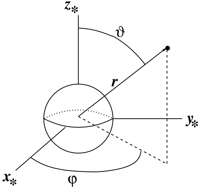
FIG. 2.—Stellar coordinate system, both Cartesian and spherical. The z_* -axis is taken as the reference direction for the field geometry. If the direction \hat{r} corresponds to the illumination ray of a scattering point at the filled circle, then \vartheta = \vartheta_i and \varphi = \varphi_i .
