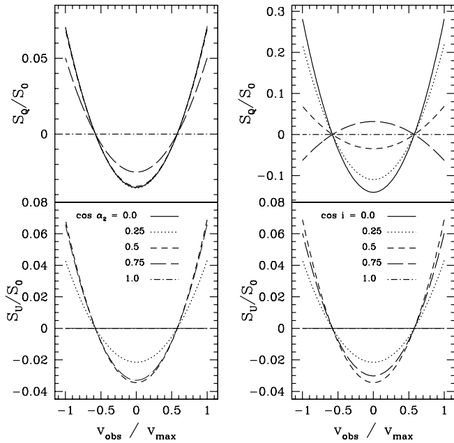
FIG. 5.—Variation of S_Q and S_U across an expanding thin spherical shell that is threaded by an axial magnetic field of constant strength. The Stokes source functions are plotted against observed Doppler shift, from the front side at v_{\text{obs}}/v_{\text{max}} = -1 to the rear side at v_{\text{obs}}/v_{\text{max}} = +1 . Left panels: For fixed \cos i = 0.5 , the effect of varying the Hanle effect via the parameter \cos \alpha_2 = 1.0, 0.75, 0.5, 0.25 , and 0.0 for B/B_H = 0.0, 0.9, 1.7, 3.9 , and \infty . Right panels: For fixed \cos \alpha_2 = 0.5 , the effect of varying the viewing inclination (with the solid line for i = 90^\circ and the dot-dashed line for i = 0^\circ ). Note that the top right panel uses a scale different from the other panels.
