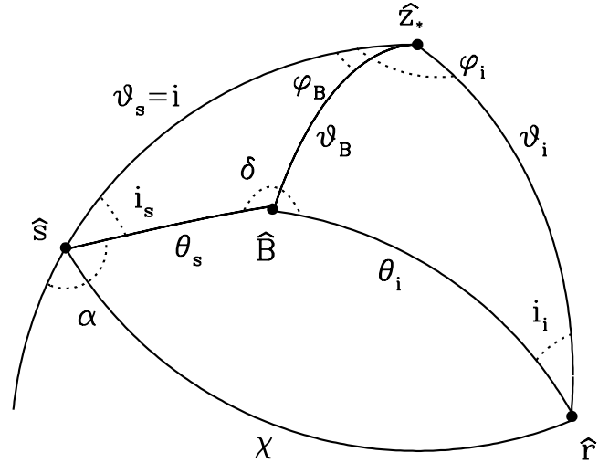
FIG. 3.—Scattering geometry centered at the scattering point of Fig. 2. The unit vectors \hat{r} and \hat{s} are for the radial direction and the scattering direction. The angles (\chi, \alpha) are polar spherical angles for the observer (along \hat{s} ). The angles \vartheta_B and \varphi_B specify the vector orientation of the local magnetic field, B . The angles (\theta, \phi) are polar spherical angles for a system defined by this local magnetic field. The angle i_s is a Mueller rotation angle that rotates the Q - and U -polarizations from the reference frame of the magnetic field to that of the observer's measurement axes.
