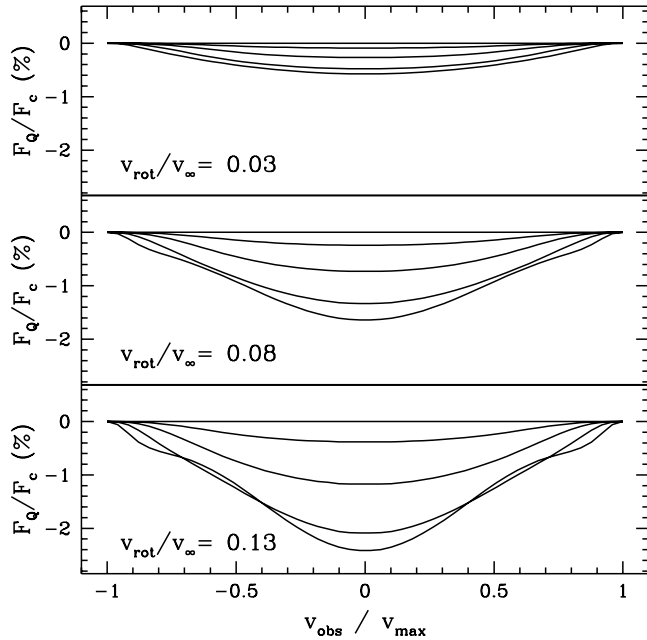
FIG. 9.—Polarized line profiles for slow magnetic rotators at three different values of v_{\text{rot}}/v_{\infty} , as indicated. The magnetic geometries are determined by the WCFields model. The wind density and flow velocity are taken to be spherical, so that the polarization arises only from the Hanle effect itself. The different curves in each panel are for Hanle ratios of B_*/B_{\text{Han}} = 0, 3, 10, 30, and 100 , with stronger polarizations resulting for larger Hanle ratios. The inclination is 90^\circ , and \tau_l = 1 . A weak U -signal exists, but we choose not to show it here.
