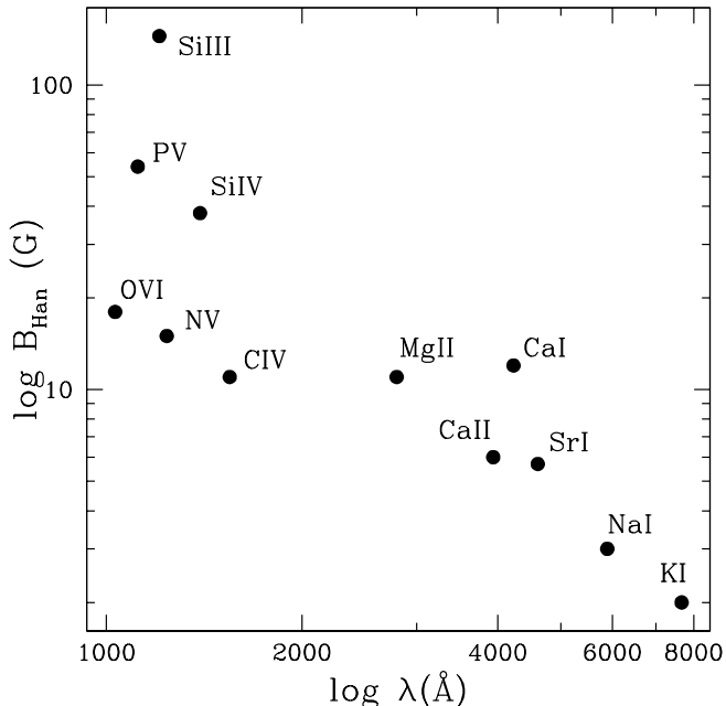
FIG. 1.—Plot of the Hanle field strength B_{\text{Han}} for resonance scattering lines common to astrophysics. Note that a few of these lines are singlets, but most are Li-like doublets. Of the doublets, only the shorter wavelength component will show a Hanle effect, since the longer wavelength component scatters isotropically and produces no line polarization. It is evident that shorter wavelength lines, having higher A -values, tend to have higher Hanle field values. The shorter wavelength lines are also associated with the more highly ionized atoms that are commonly observed in hot star winds.
