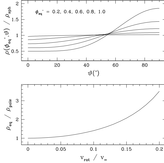
FIG. 16.—Wind geometry of WCZ models using our approximations for slowly rotating stars. Top : Variation of the normalized wind with density latitude \vartheta at different values of \phi'_{\text{eq}} . Bottom : Asymptotic wind density contrast between the equator and the pole as a function of the stellar rotation normalized to the wind terminal speed.
