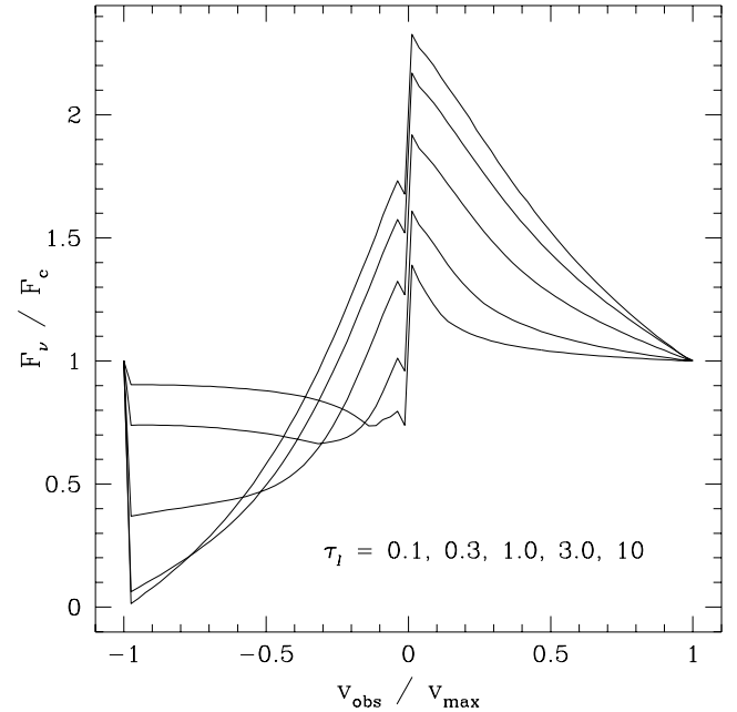
FIG. 4.—Sequence of P Cygni profiles produced by our code using the escape probability method with volume emissivity. The profiles are for optical depth scales \tau_l as indicated, with thicker lines producing deeper blueshifted absorption and stronger redshifted emission. The dip that appears just blueward of line center in these profiles is real. In each case the wind velocity law is with \gamma = 1 and for an ion species of constant ionization fraction.
