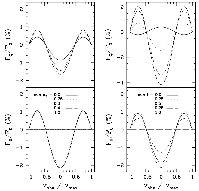
FIG. 6.—Results for the Q and U polarized flux profiles from our numerical code for an axial magnetic field of constant strength with \tau_l = 1.0 and \gamma = 1 . The sequence of line types is the same as in Fig. 5, but the values used for \cos \alpha_2 have been changed slightly so that the profiles can more easily be seen. The left panels are for \cos i = 0.5 with different \alpha_2 values, and the right panels are for \cos \alpha_2 = 0.3 , but for different values of i . The vertical scale is different for the top right panel. The integrated polarized line flux in both Q and U is generally nonzero.
