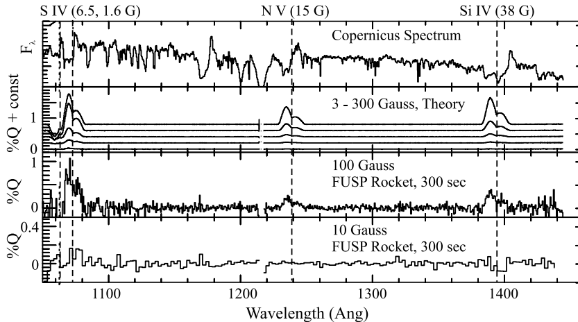
Figure 1. A simulated FUSP observation of \zeta Ori. Top: Copernicus spectrum. Second panel: theoretical polarization profiles for three resonance lines, B_{Han} listed at top. Bottom panels: simulated 300 sec FUSP observations for base wind fields of 100 Gauss (unbinned) and 10 Gauss (binned to 2.4\text{\AA} )
